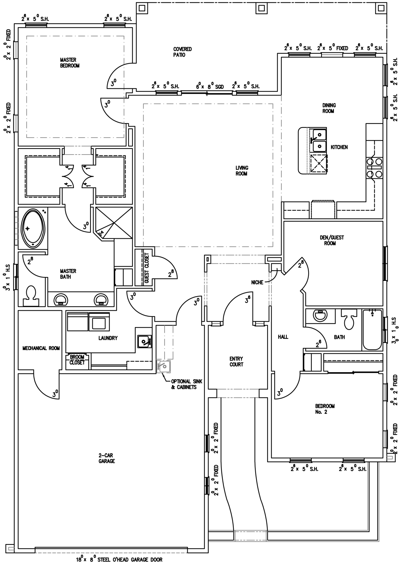
1670 fFLOOR PLAN
